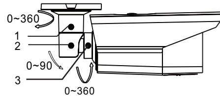
Figure 2-8 3-axis Adjustment
