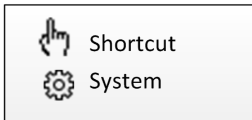
Figure 4-21 Menu
